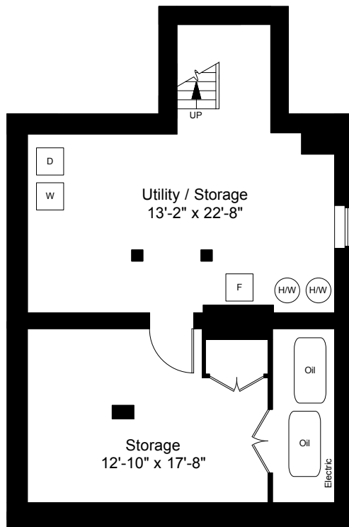
Basement Plan Ceiling Height = 6'-6"
