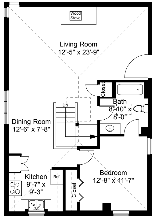
Carriage House - Second Floor Plan Ceiling Height = 10'-4"
