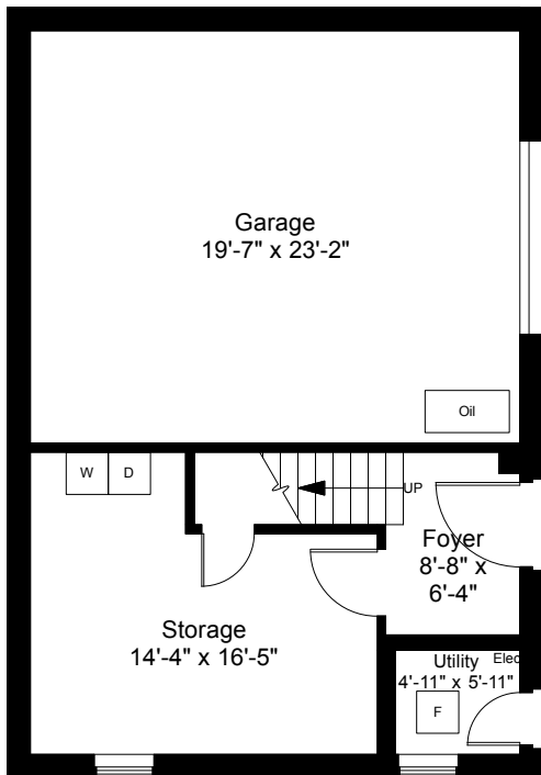
Carriage House - First Floor Plan Ceiling Height = 8'-10"
