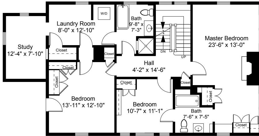
Second Floor Plan Ceiling Height = 8'-1"
