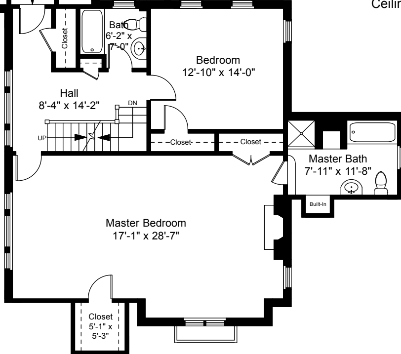
Second Floor Plan Ceiling Height = 8'-2"
