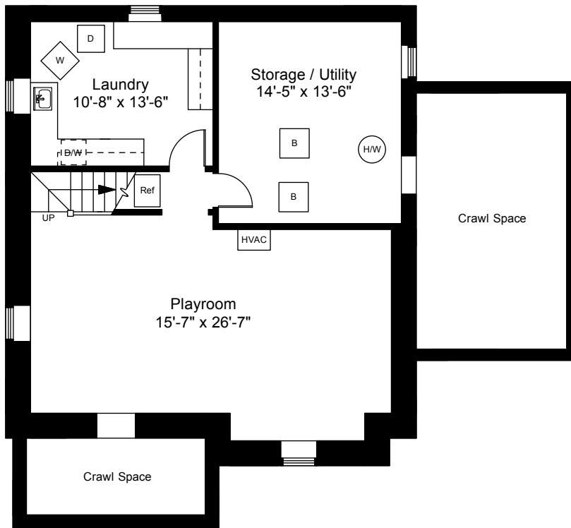
Lower Level Plan Ceiling Height = 7'-3"
