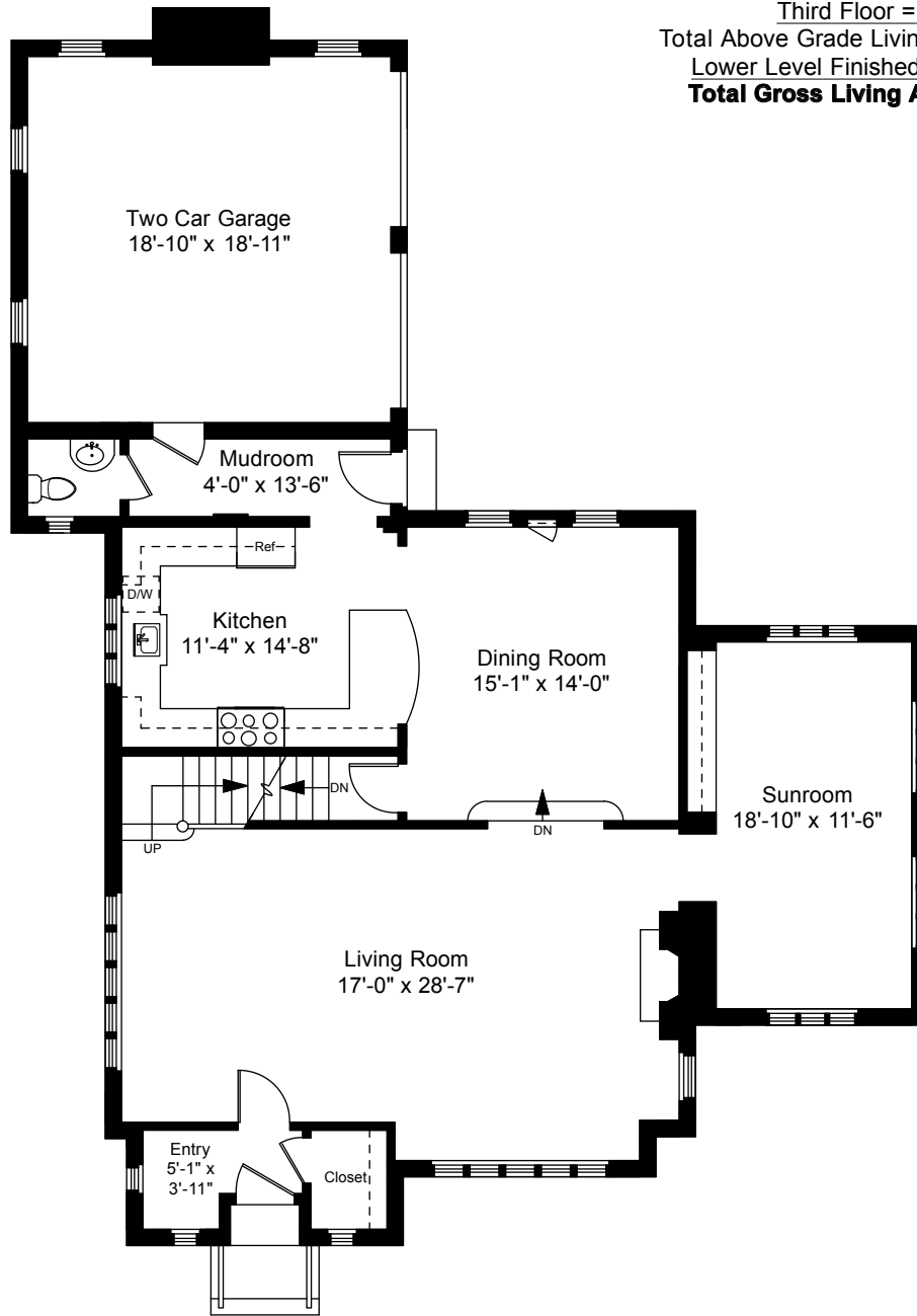
First Floor Plan Ceiling Height = 8'-4"
