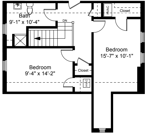
Third Floor Plan Ceiling Height = 8'-0"
