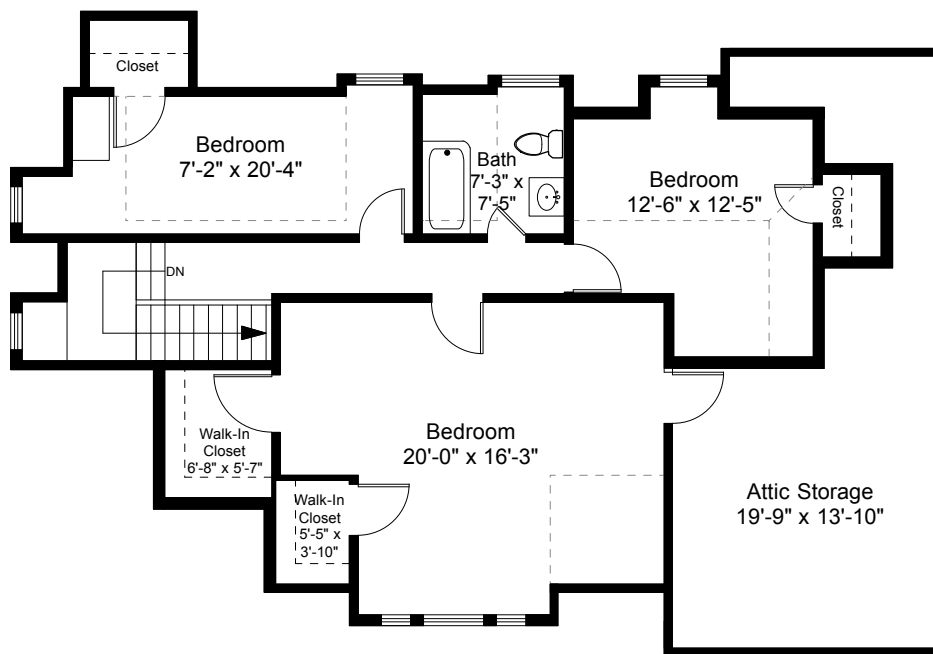
Third Floor Plan Ceiling Height = 7'-11"
