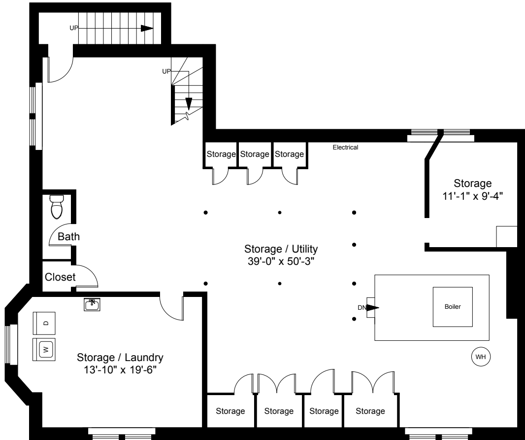
Basement Plan Ceiling Height = 8'-7"
