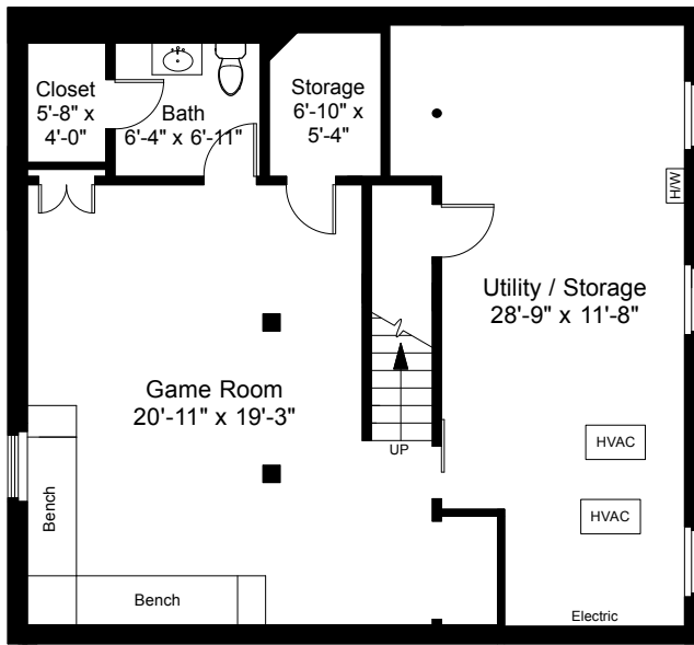
Lower Level Plan Ceiling Height = 7'-0"
