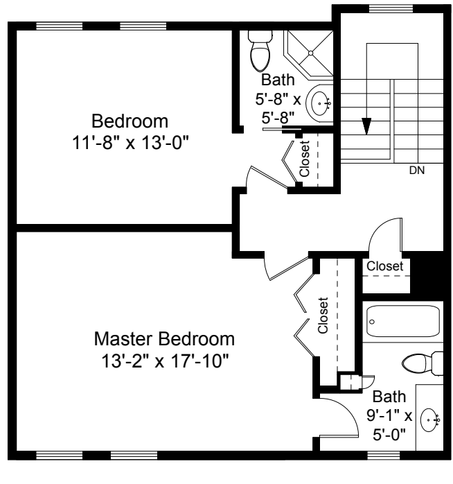
Second Floor Plan Ceiling Height = 8'-0"
