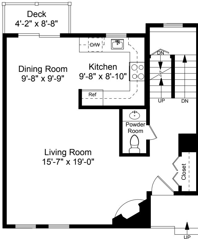
First Floor Plan Ceiling Height = 8'-0"
