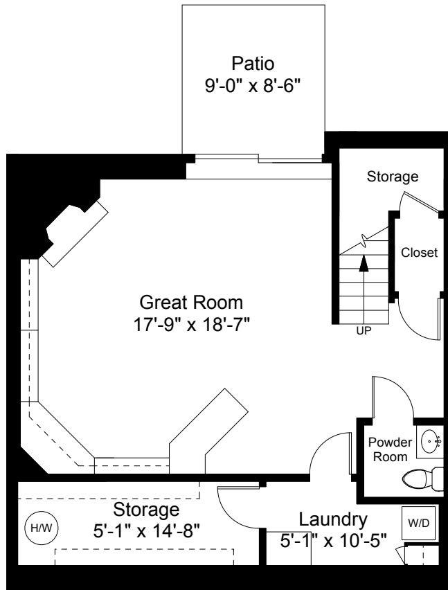
Lower Level Plan Ceiling Height = 7'-10"
