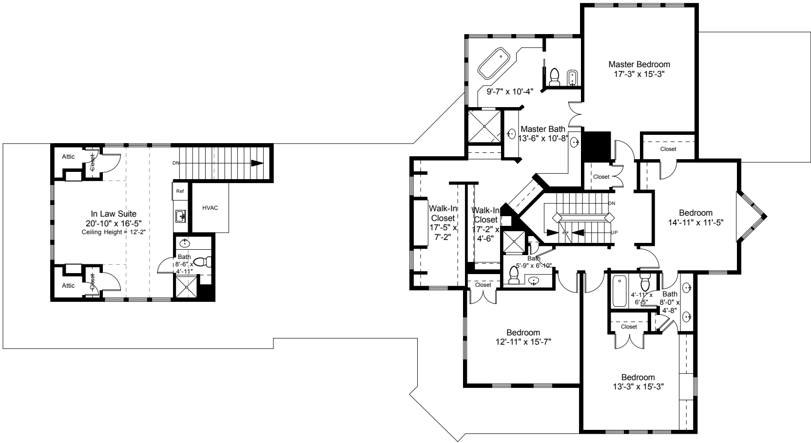
Second Floor Plan Ceiling Height = 8'-4"
