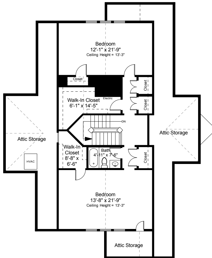
Third Floor Plan Ceiling Height = 7'-10"
