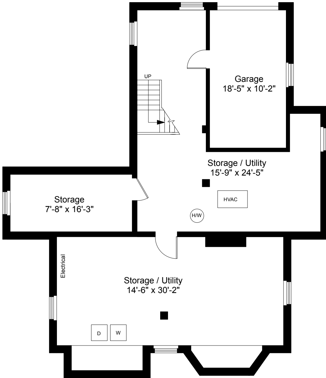
Basement Plan Ceiling Height = 7'-6"
