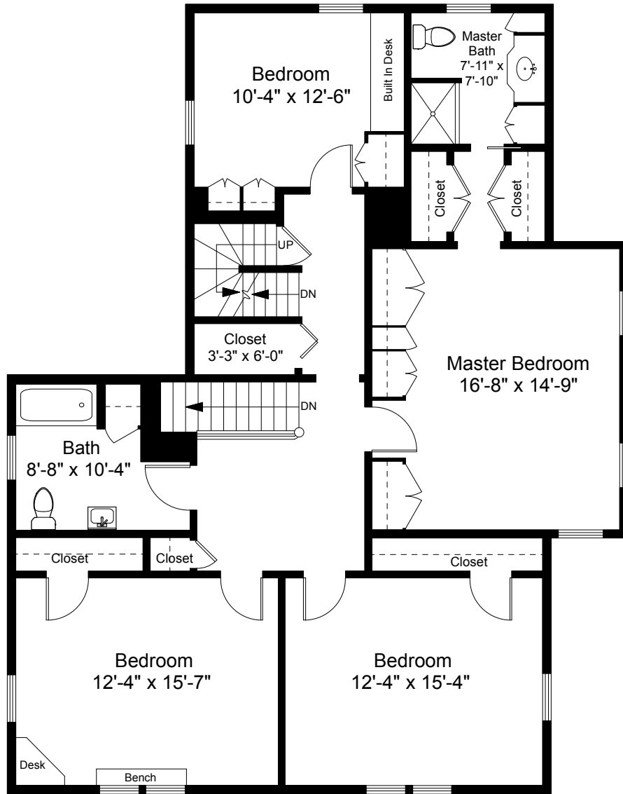
Second Floor Plan Ceiling Height = 8'-6"
