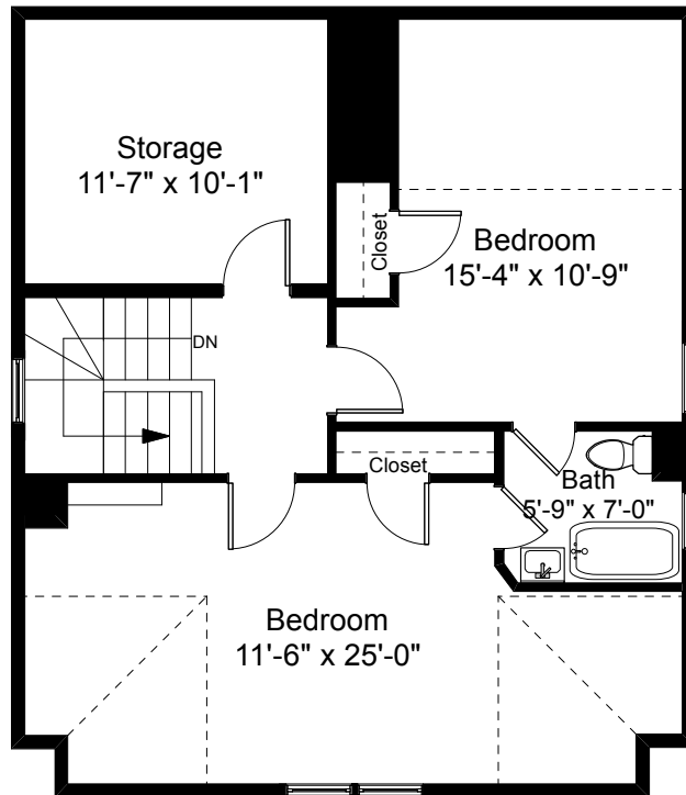
Third Floor Plan Ceiling Height = 8'-4"
