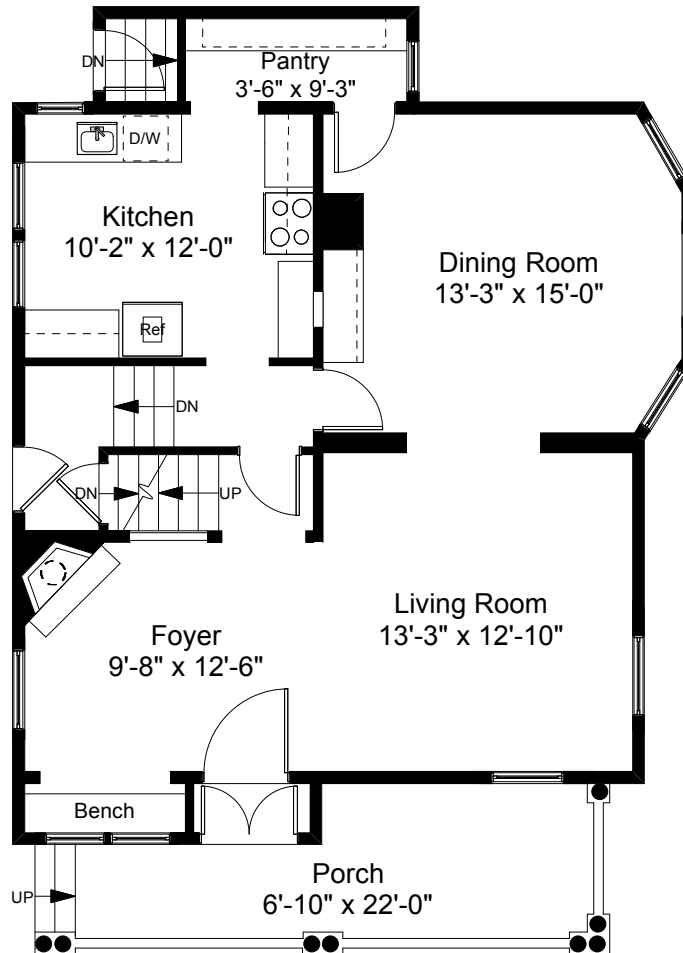
First Floor Plan Ceiling Height = 8'-8"
