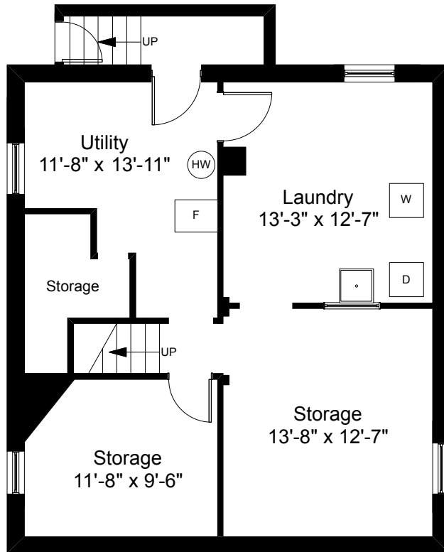
Basement Plan Ceiling Height = 7'-4"
