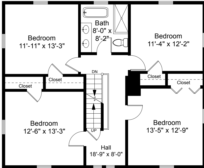
Second Floor Plan Ceiling Height = 8'-6"
