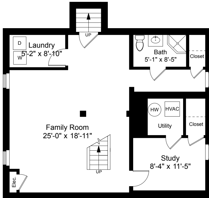
Lower Level Plan Ceiling Height = 7'-3"
