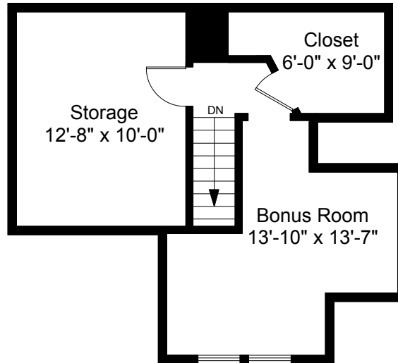
Third Floor Plan Ceiling Height = 8'-4"
