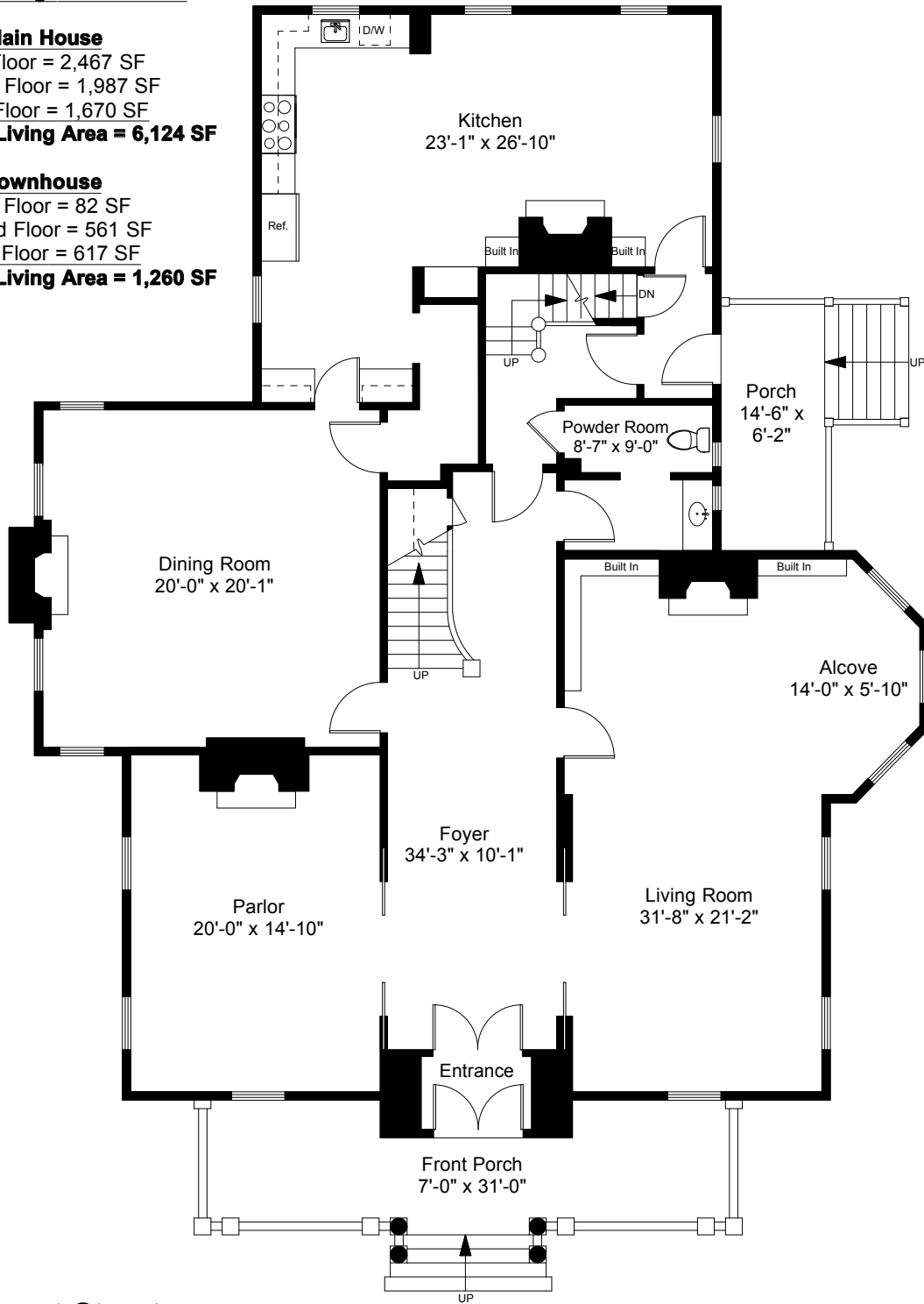
First Floor Plan Ceiling Height = 11'-6"
