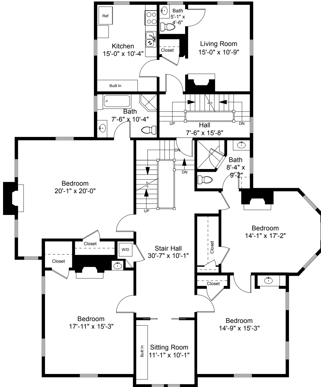
Second Floor Plan Ceiling Height = 10'-6"
