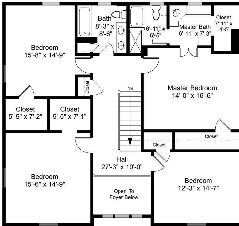
Second Floor Plan Ceiling Height = 8'-0"
