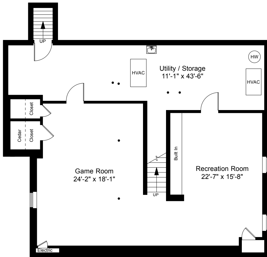
Lower Level Plan Ceiling Height = 7'-4"
